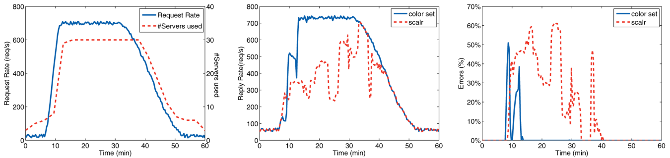
Fig. 7. Left figure: request rate and #servers used. Middle and right figures: comparison with Scalr.
