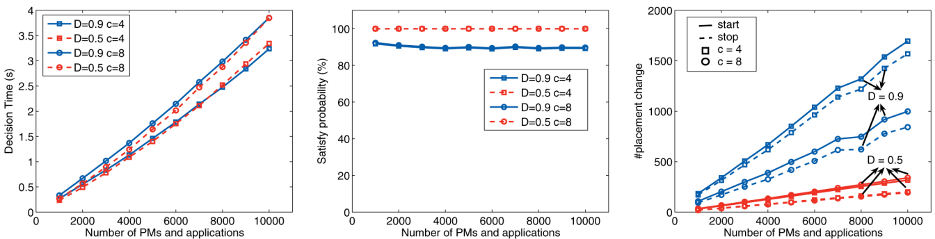
Fig. 11. Scalability of the algorithm as the number of servers and applications increases.
