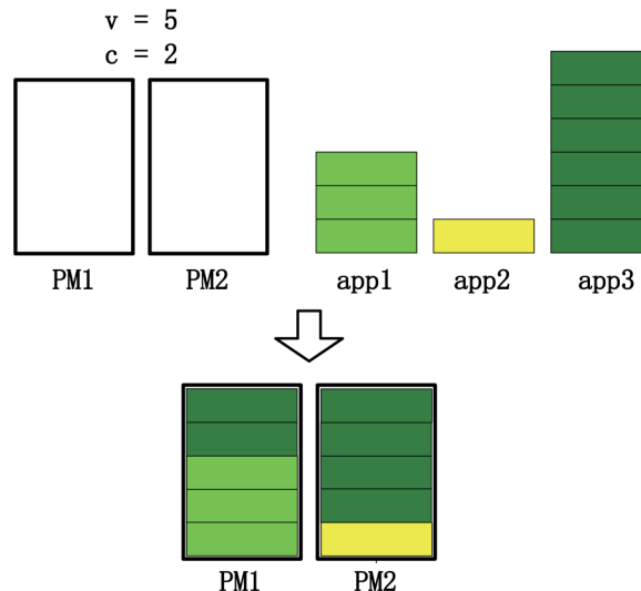
Fig. 3. Class constrained bin packing (CCBP).
