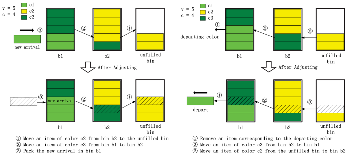
Fig. 4. Arrival of a new item (left) and departure of an existing item (right).
