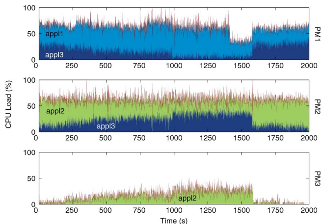
Fig. 6. Load shifting to avoid placement change.
