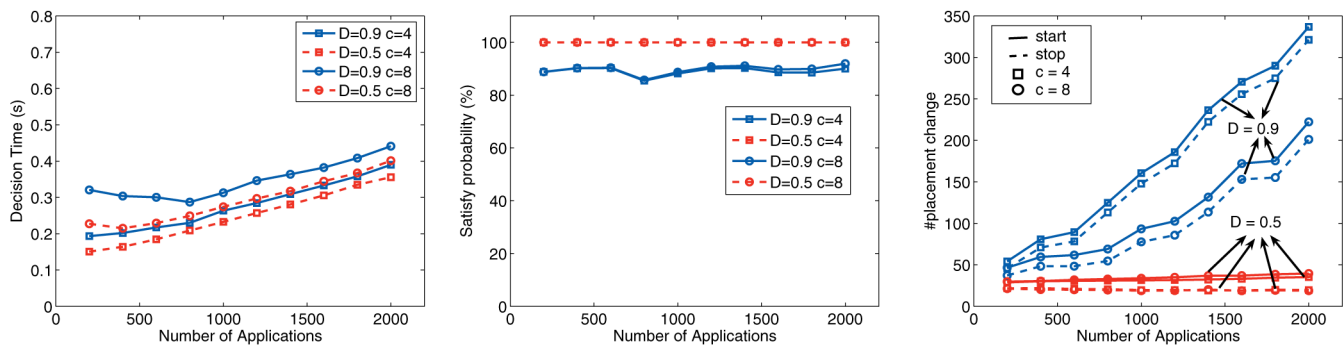
Fig. 12. Performance of the algorithm as the number of applications increases.
