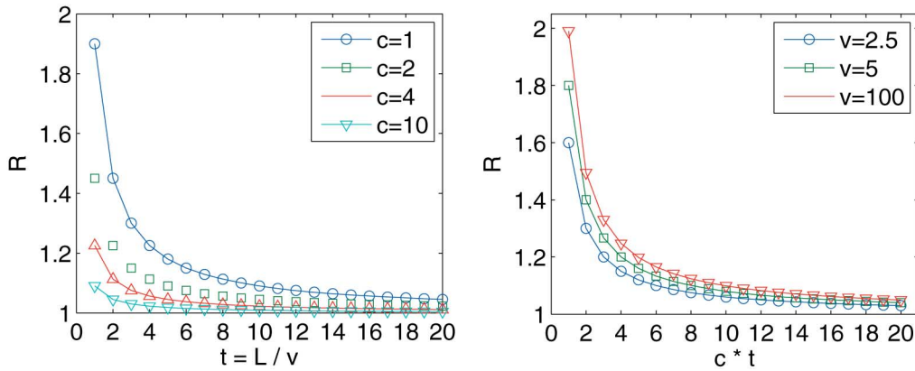
Fig. 5. Approximation ratio as the parameters change.
