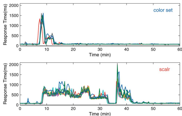
Fig. 8. Comparison of the response time.
