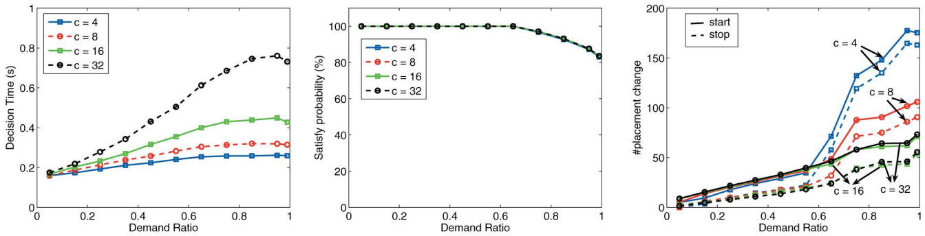
Fig. 10. Performance of the algorithm as the demand increases.
